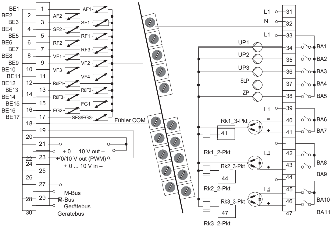
Fig. 11: Connection of the EQJW246F002 Controller
